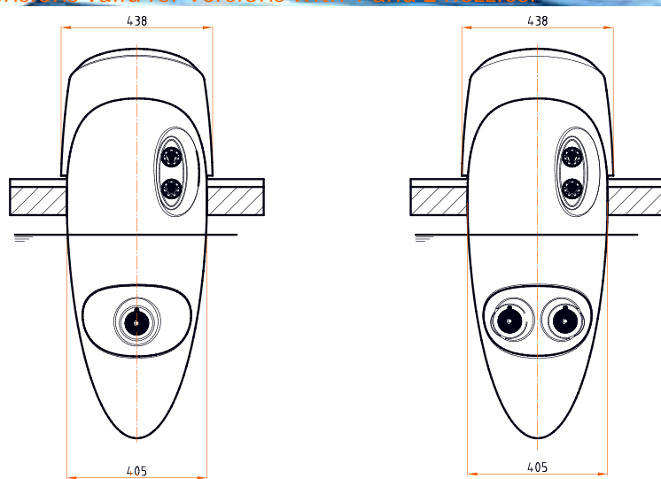
Dimensioned draw (in mm) Dimensions valid for versions with 1 and 2 nozzles.
